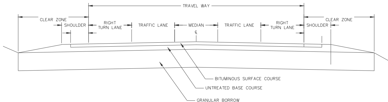
Figure A-7 Typical Cross Section
